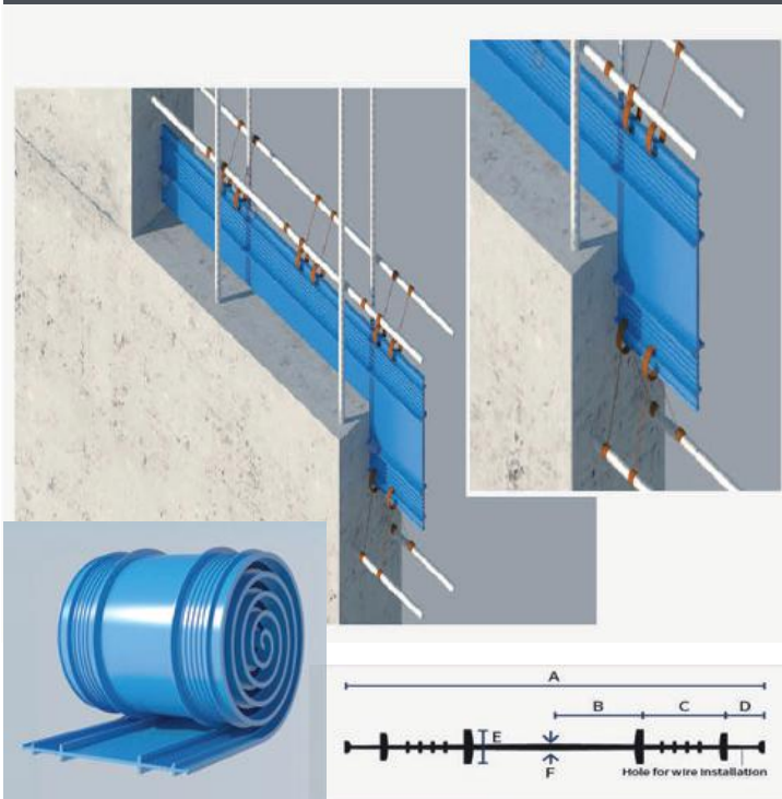
WATERSTOP
