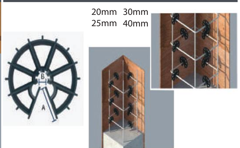
WHEEL SPACER
